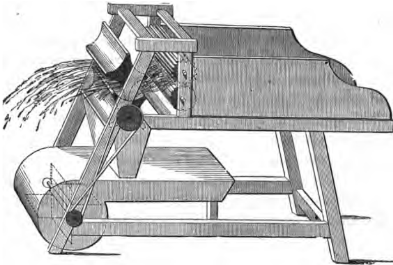
JUBB'S THRASHING-MACHINE.
